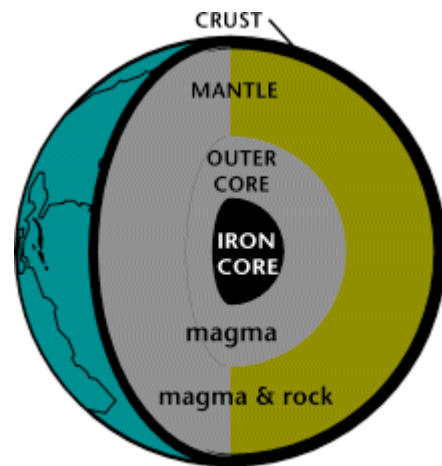
THE EARTH'S INTERIOR
