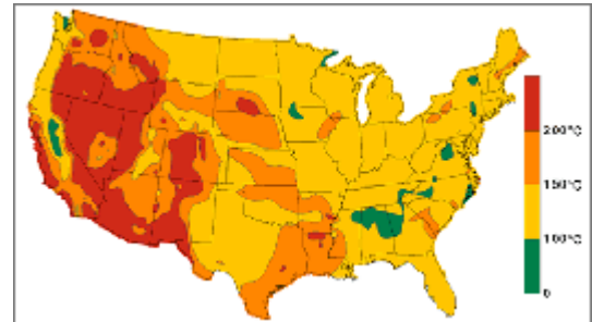
U.S. Geothermal Resource Map
