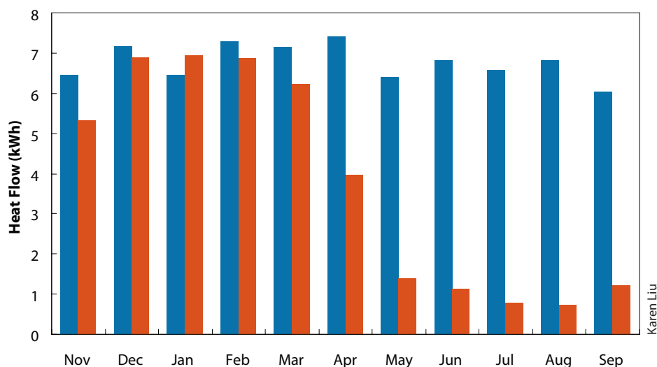
Figure 8: Comparison of Average Daily Energy Demand Due to Heat Flow Through an Extensive Green versus Conventional Roof in Ottawa, Canada 17
